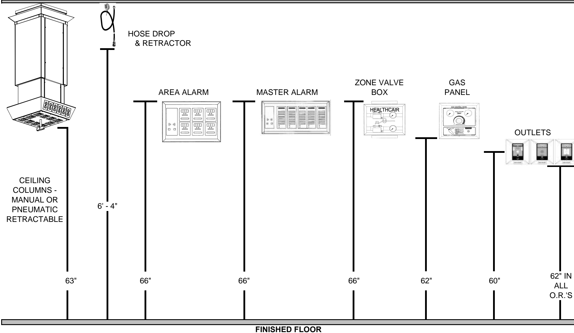
MEDICAL GAS EQUIPMENT MOUNTING HEIGHT DETAIL
